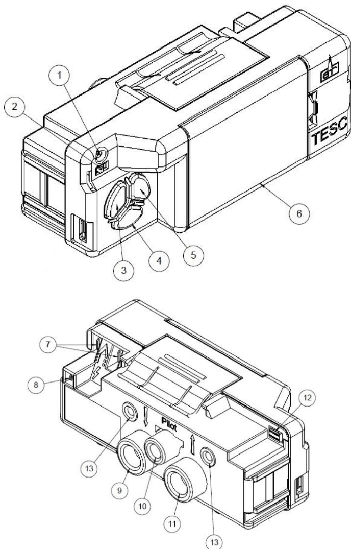
Fig 17 - Control unit
