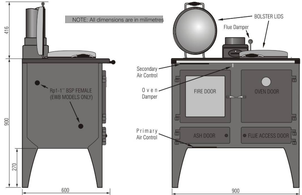
Fig. 1 - The Cooking Stove
