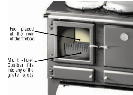
Fig. 3b - Multi-fuel version. Alternative flue bar posi-
