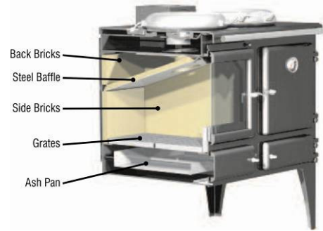
Fig. 3a - Multi-fuel version. Firebox parts
