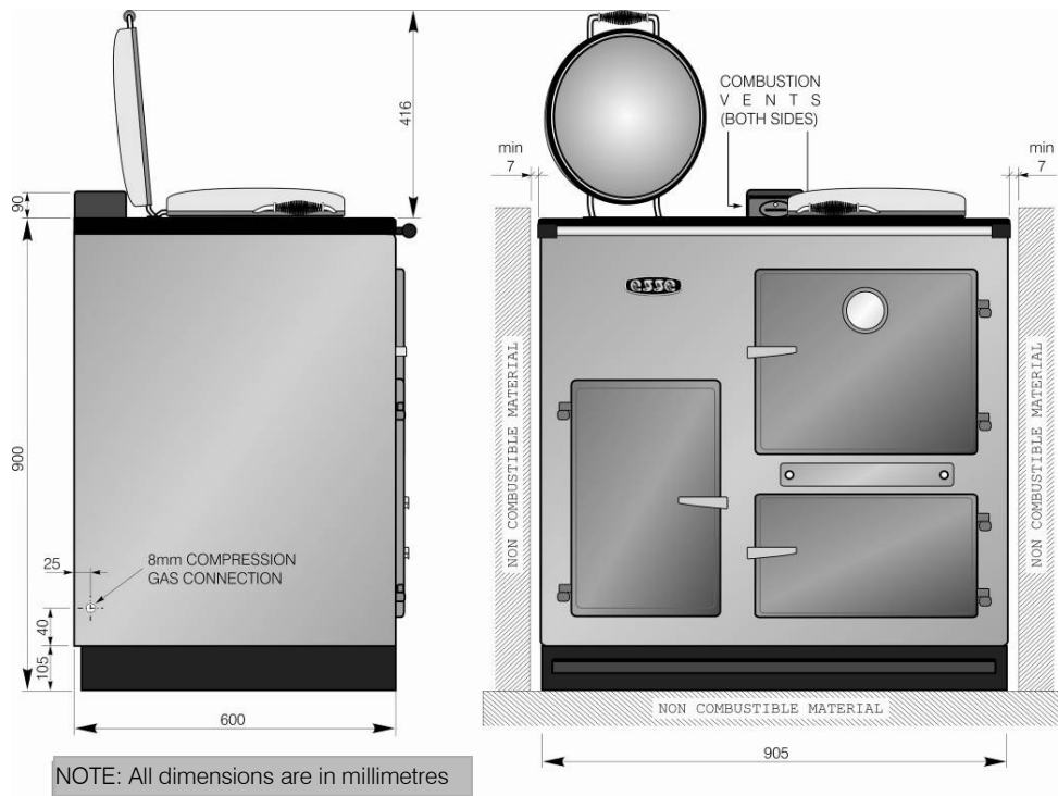
Fig. 1 - Your Cooker
