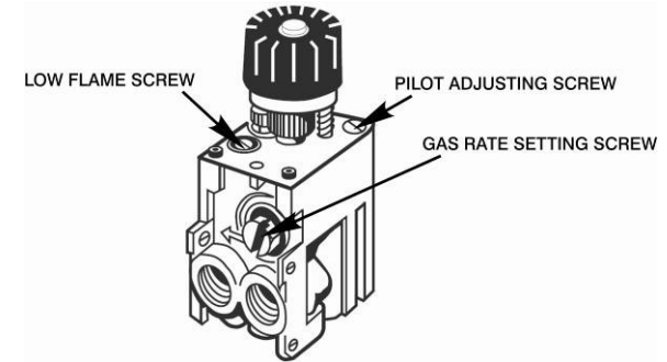
Fig. 7 - Gas Components - Schematic Arrangement
