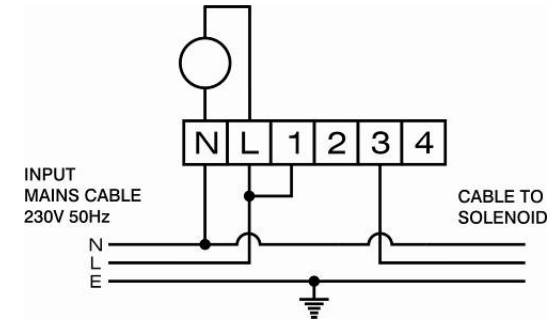
Fig. 3 - Wiring Instructions for Horstmann Electronic Timer
