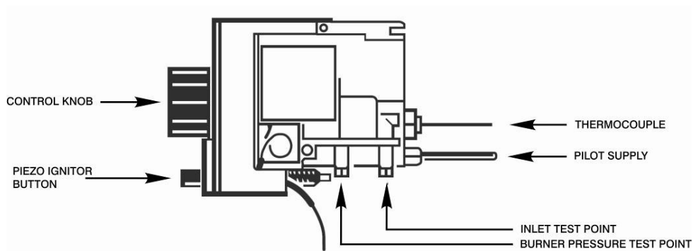
Fig. 5 - Eurosit Control Valve (Side view)
