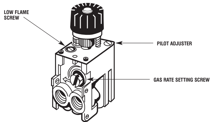
Eurosit Control Connections and Rate Screws - Fig.7
