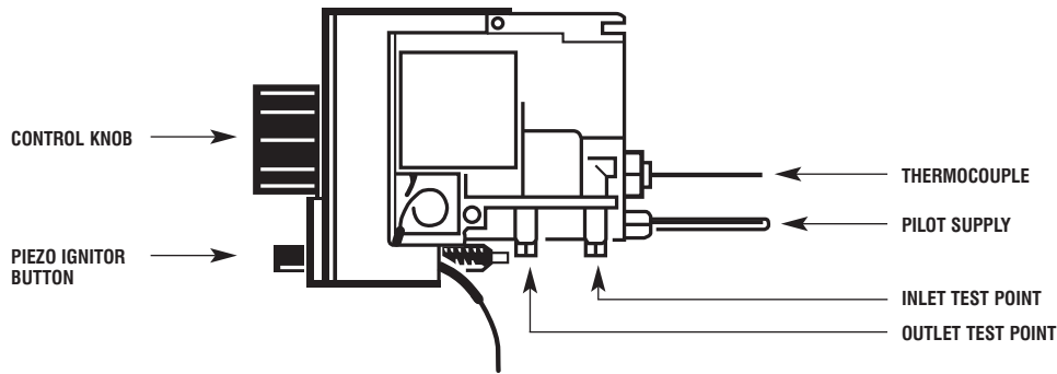
Eurosit Control Connections and Rate Screws - Fig.7
