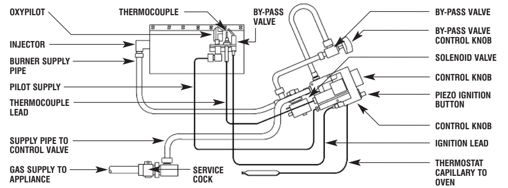
Breakdown of Burner Assembly - Fig.9
