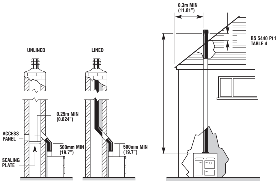
Connection to Brick Chimney - Fig.1
